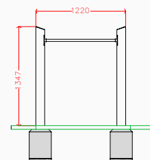
Side elevation
