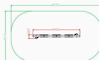
Plan elevation
