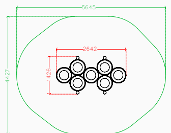
Plan elevation
