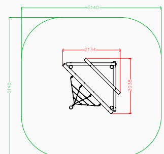
Plan elevation
