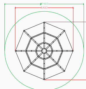
Plan elevation
