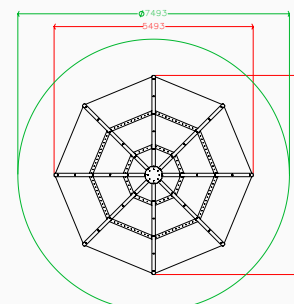
Plan elevation
