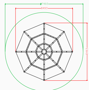
Plan elevation
